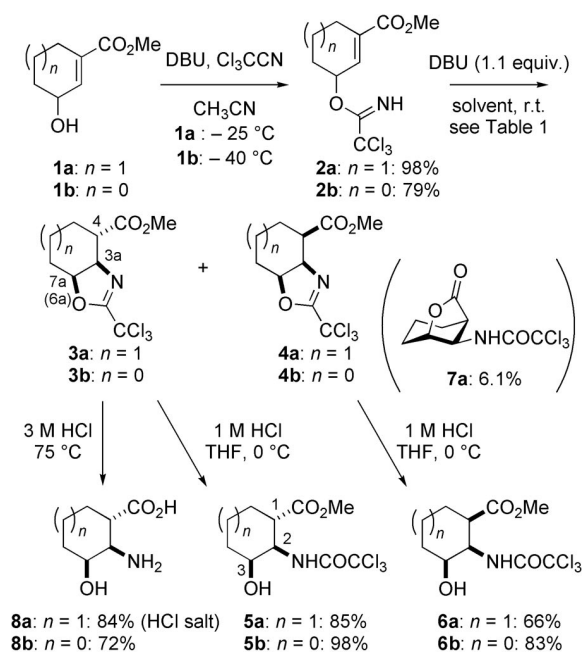
Scheme 1. Synthesis of 3-hydroxy-ACHC and -ACPC.
