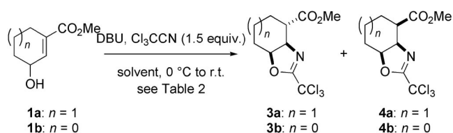
Scheme 2. One-pot synthesis of oxazolines 3a,b from allylic alcohols 1a,b .
